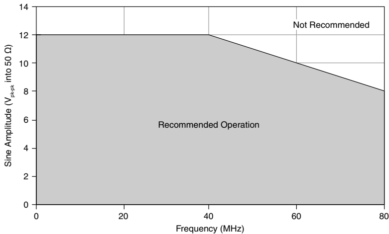
Figure 11. Amplitude Versus Recommended Sine Wave Frequency
