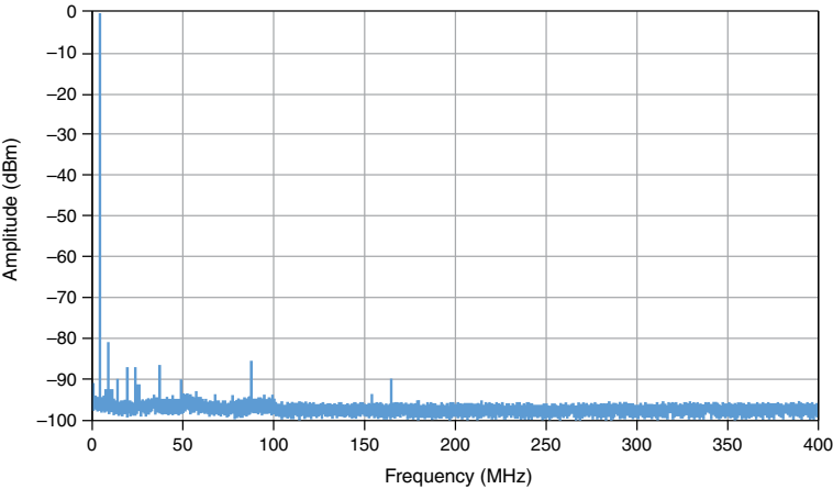
Figure 2. 5 MHz Spectrum 15 at 0.6 V pk-pk , Measured
