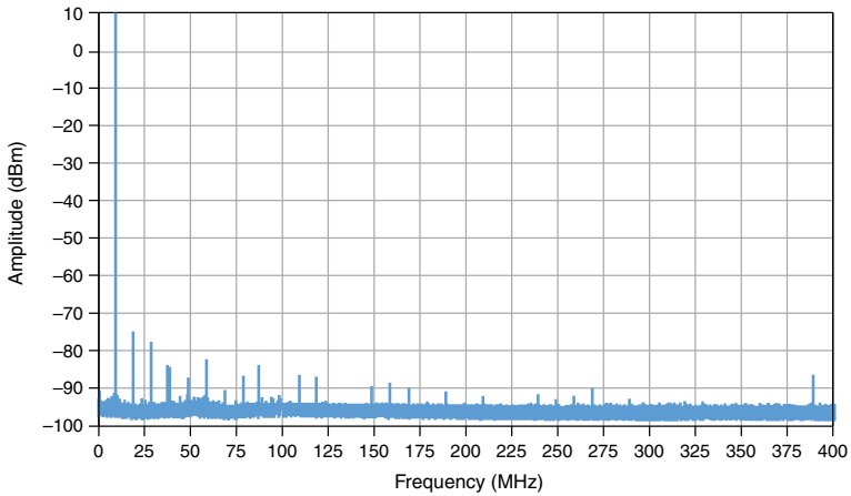
Figure 9. 10 MHz Single-Tone Spectrum 25 , Measured
