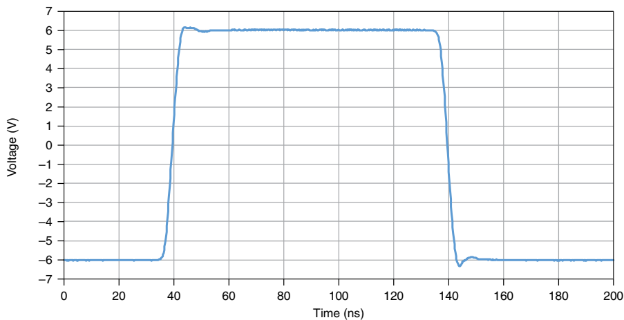
Figure 7. Square Waveform Step Response at 12\text{ V}_{\text{pk-pk}} , Measured
