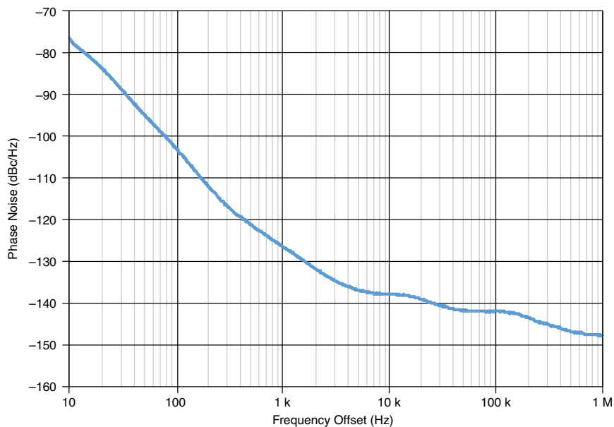
Figure 5. Phase Noise 17 , Measured
