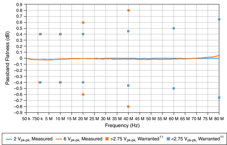
Figure 1. Passband Flatness
